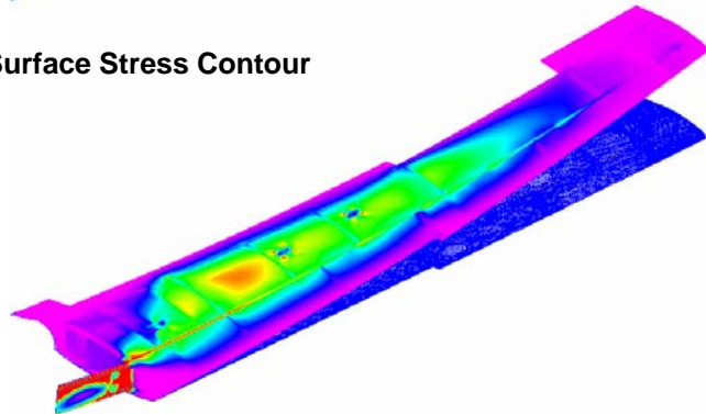
Bottom Surface Stress Contour
